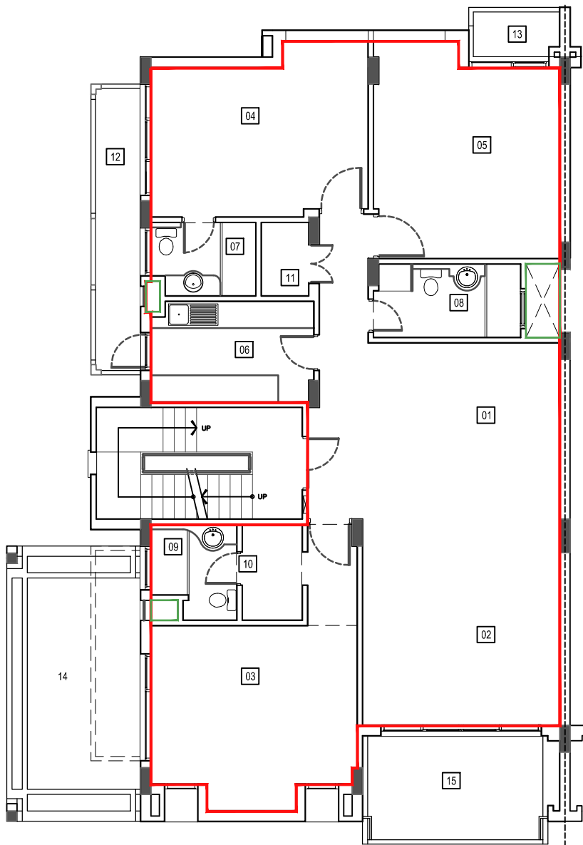
FIRST FLOOR
