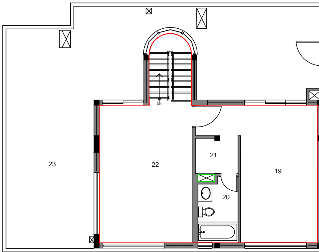
UPPER FLOOR
