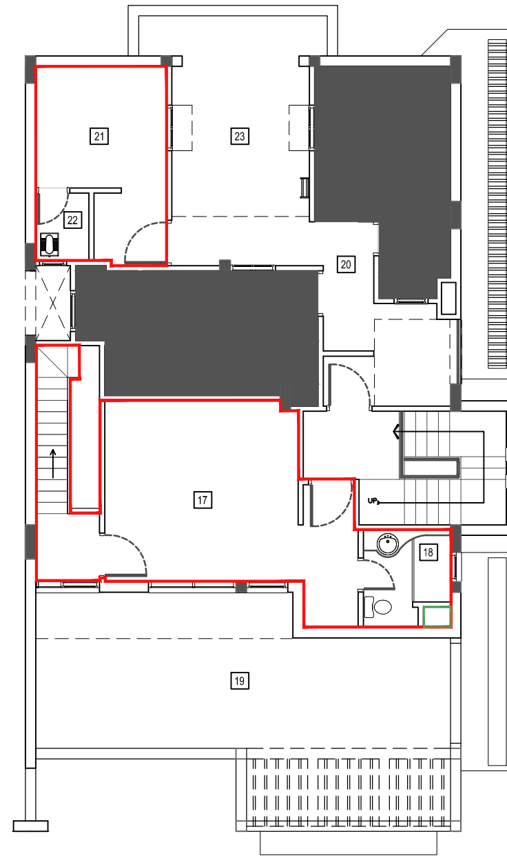
THIRD FLOOR + UTILITY AREA
